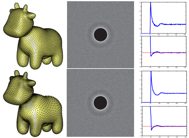
Fig. 3. Surface samplings of a cow model, with uniform (top, 4500 samples) and adaptive (bottom, 6000 samples) point distributions. On the right we show the respective plots of differential domain analysis (DDA) [54].
