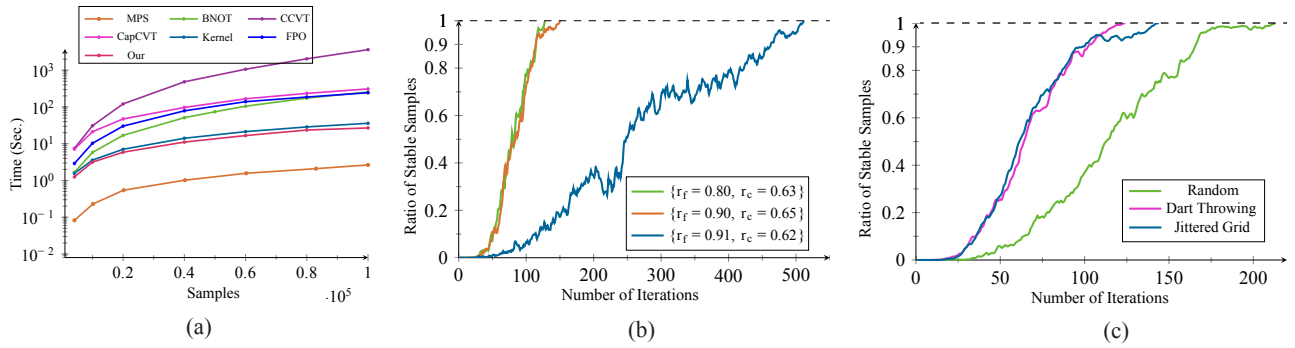
Fig. 4. Performance and convergence analysis. (a) Running time (in log scale) dependency on the number of points. (b) Convergence curves of our method with different parameter configurations. (c) Convergence curves of our method with the same parameters, but using different initialization methods.
