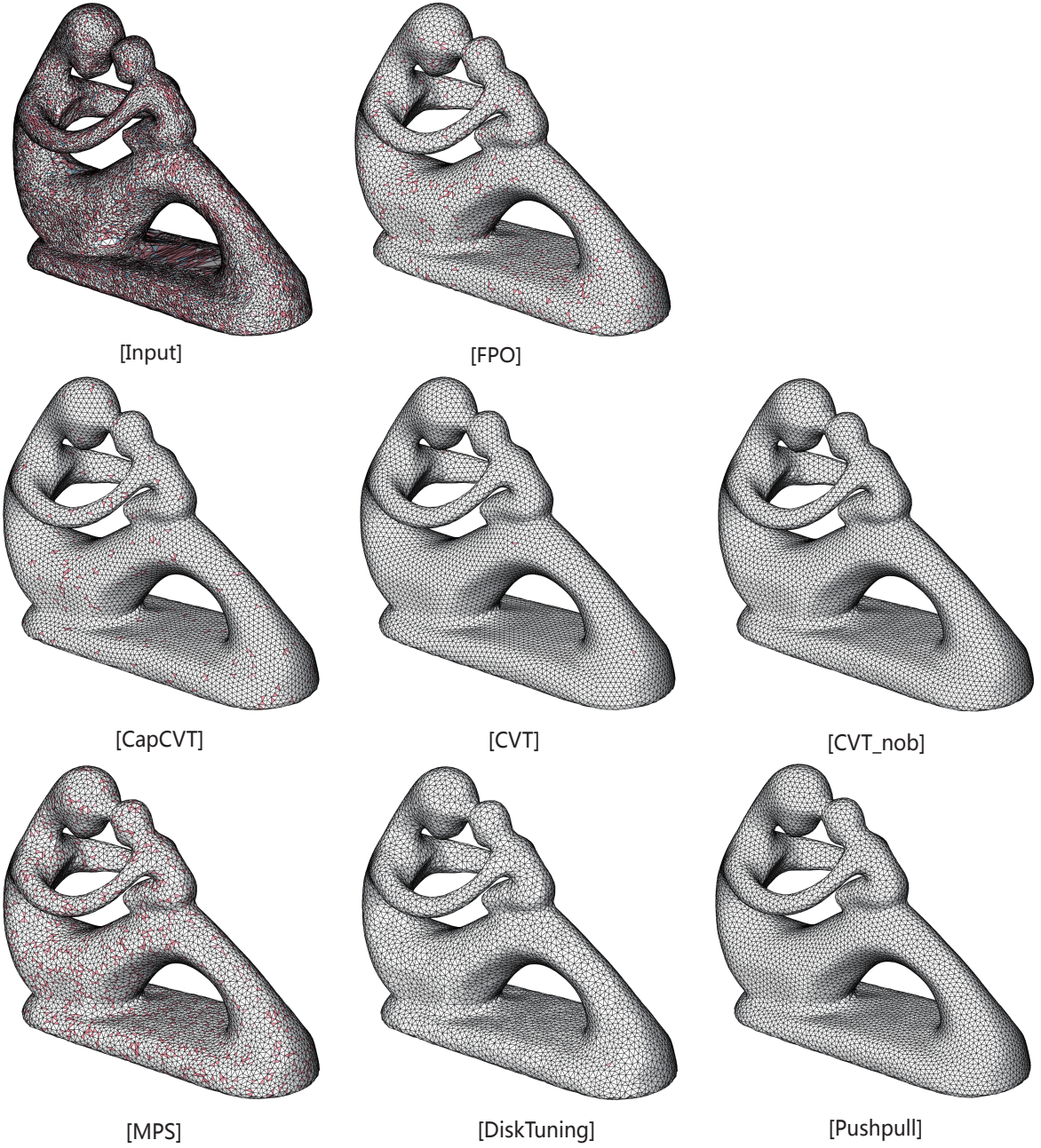
Fig. 6. Uniform remeshing results of the Fertility model. The obtuse triangles are shown in pink, and triangles with \theta_{min} < 30 are shown in blue.
