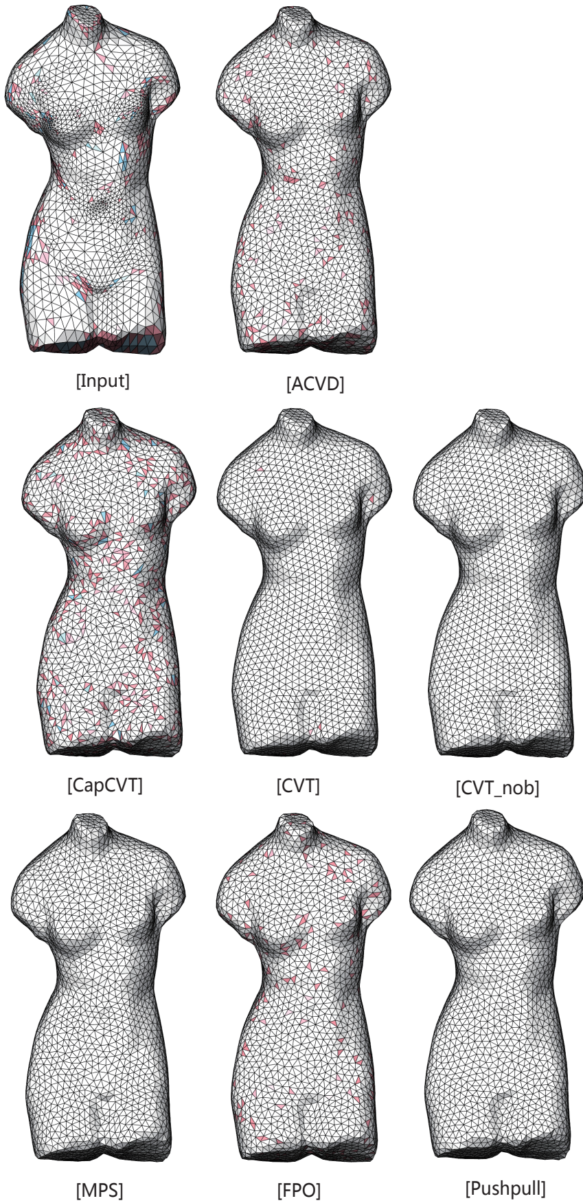
Fig. 4. Uniform remeshing results of the Venus model. The obtuse triangles are shown in pink, and triangles with \theta_{min} < 30 are shown in blue.
