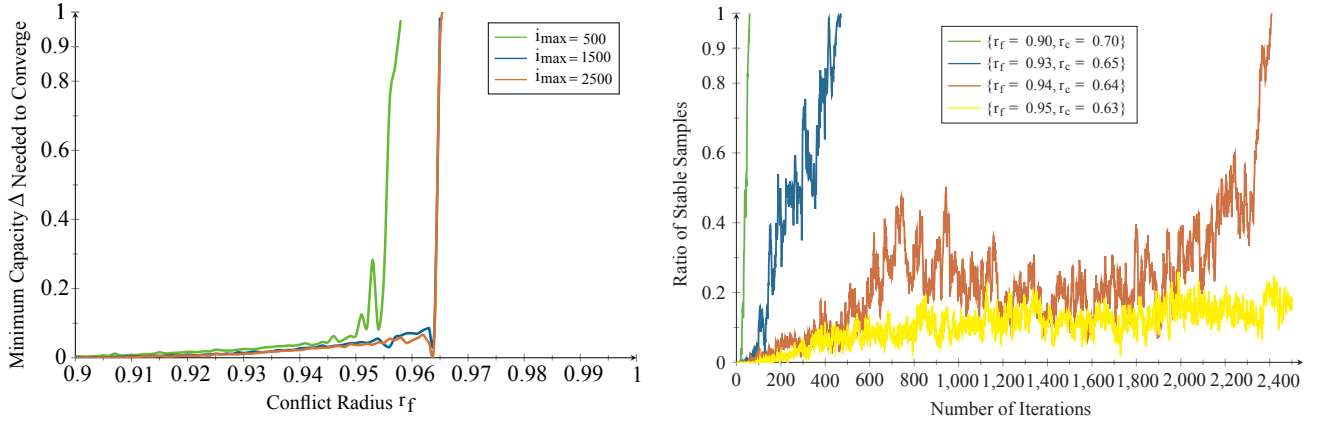
(a) The evolution of the minimum \Delta that is required for the algorithm to converge.
