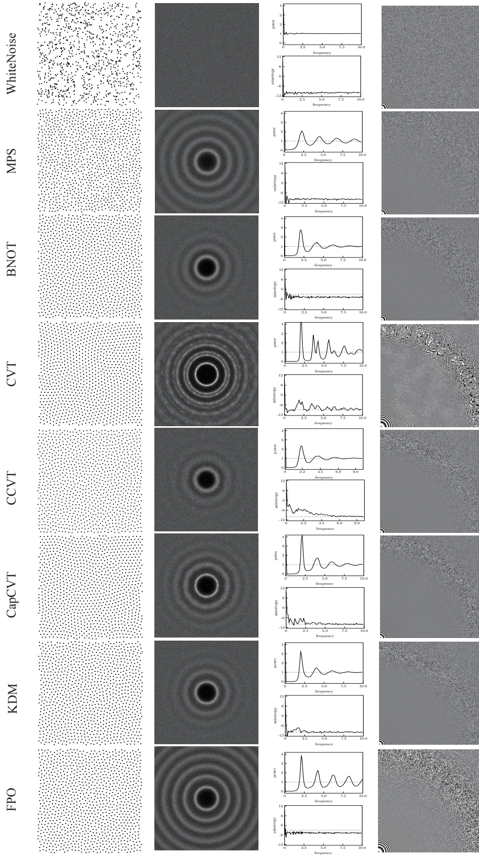
Fig. 2. Spectral and anti-aliasing analysis of previous blue noise methods. From left to right: distribution of 1024 points, power spectrum, radial means (top) and anisotropy (bottom), zone plate test function sampled by 512^2 points.
