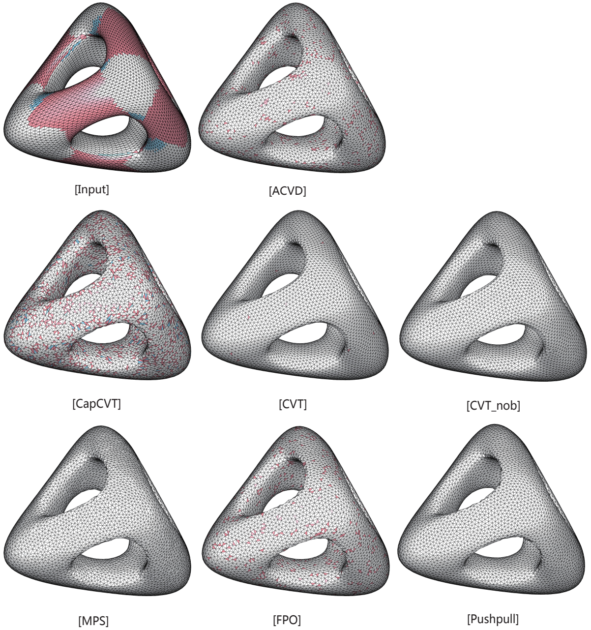
Fig. 5. Uniform remeshing results of the Genus model. The obtuse triangles are shown in pink, and triangles with \theta_{min} < 30 are shown in blue.
