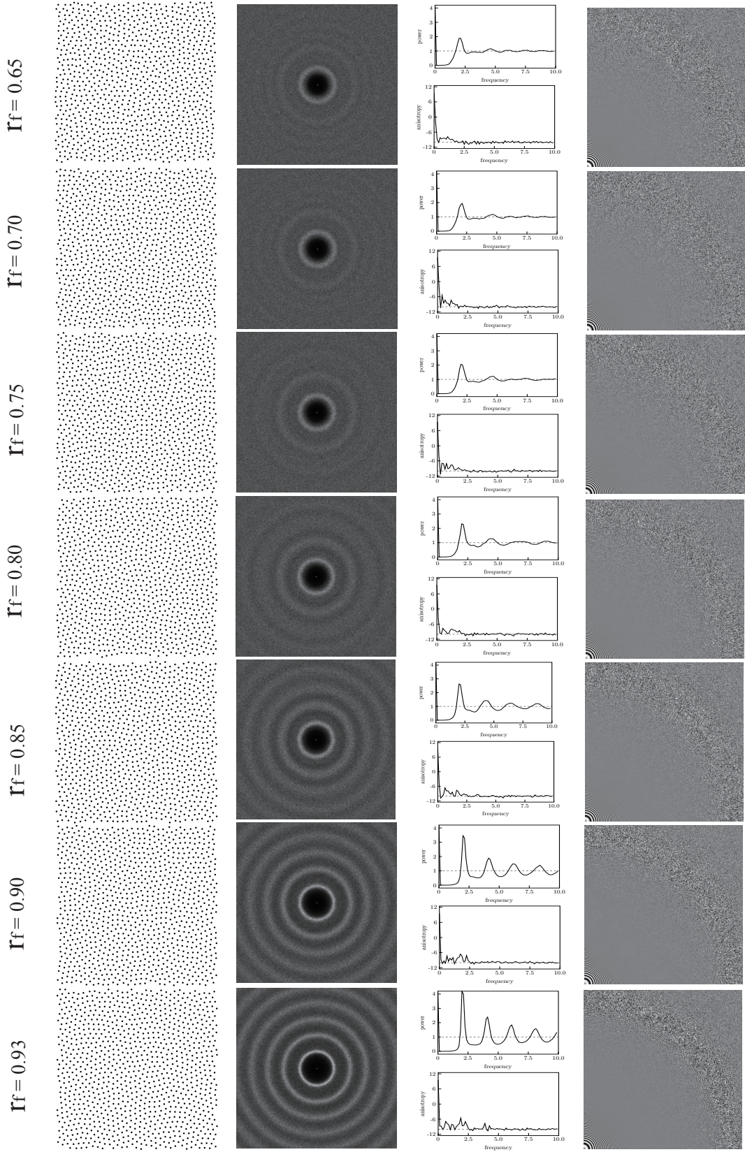
Fig. 3. Spectral and anti-aliasing analysis of our algorithm with fixed r_c = 0.67 . From left to right: distribution of 1024 points, power spectrum, radial means (top) and anisotropy (bottom), zone plate test function sampled by 512^2 points.
