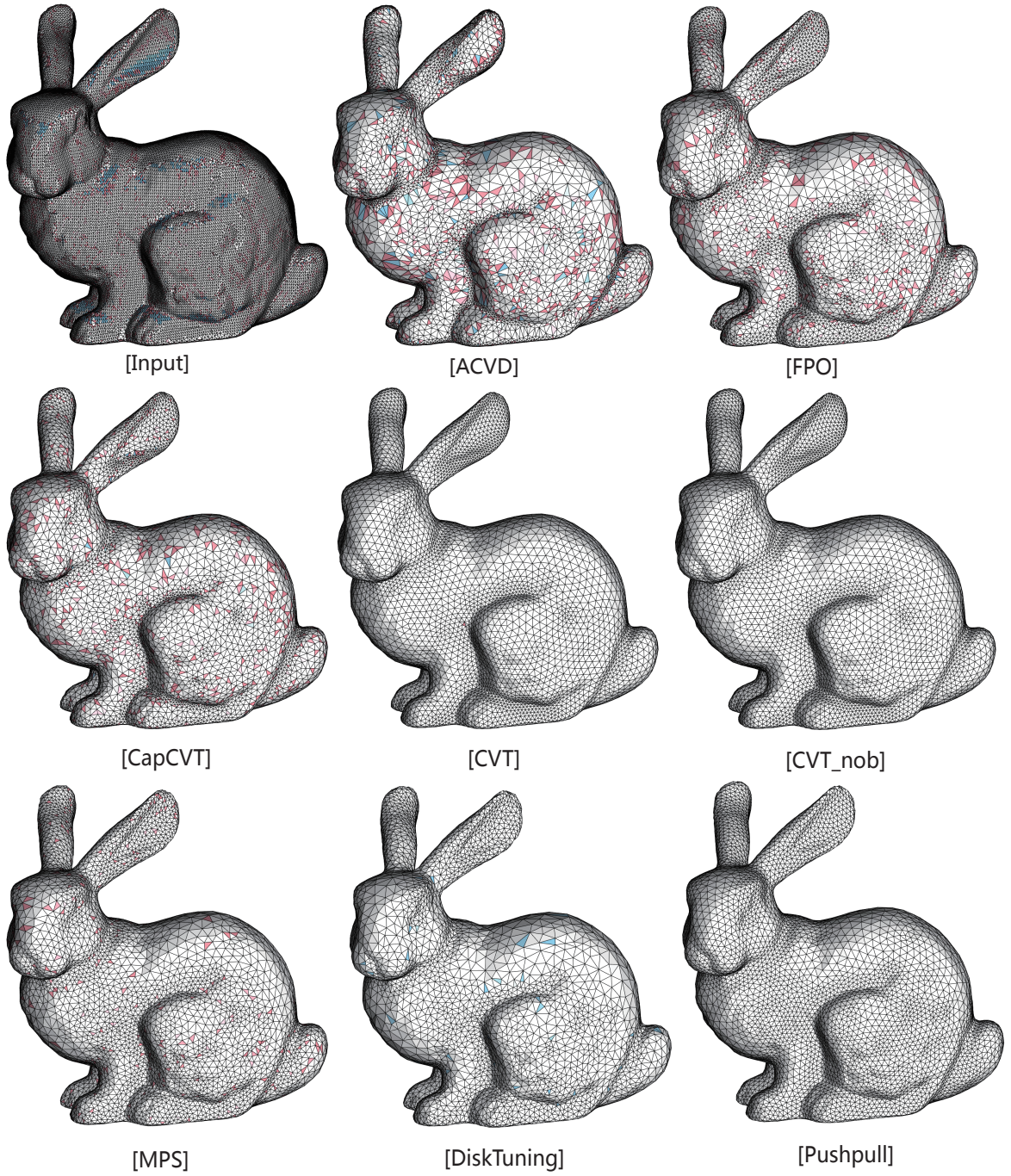
Fig. 8. Adaptive remeshing results of the Bunny model. The obtuse triangles are shown in pink, and triangles with \theta_{min} < 30 are shown in blue.
