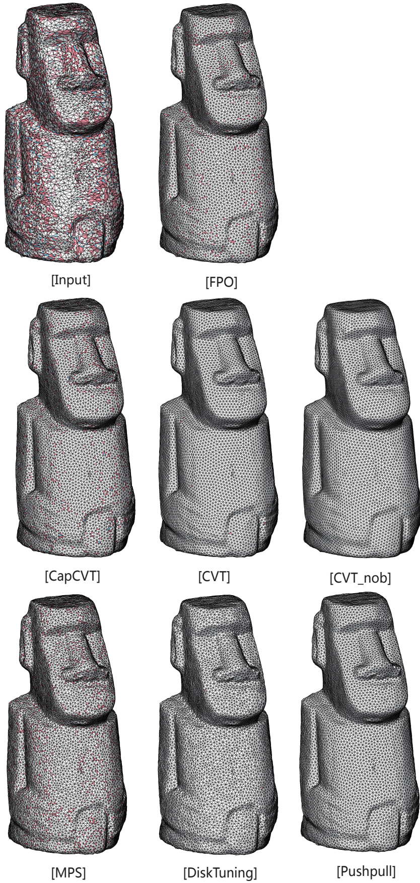
Fig. 7. Uniform remeshing results of the Moai model. The obtuse triangles are shown in pink, and triangles with \theta_{min} < 30 are shown in blue.
