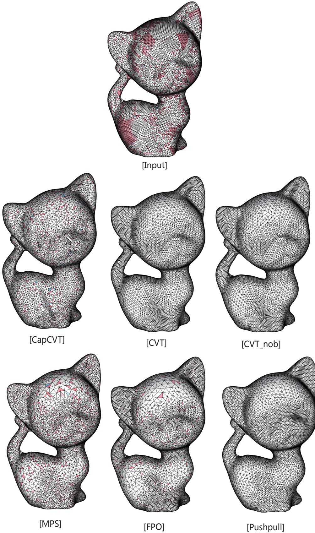
Fig. 10. Adaptive remeshing results of the Kitten model. The obtuse triangles are shown in pink, and triangles with \theta_{min} < 30 are shown in blue.
