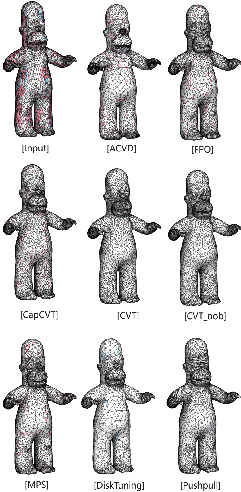
Fig. 9. Adaptive remeshing results of the Homer model. The obtuse triangles are shown in pink, and triangles with \theta_{min} < 30 are shown in blue.
